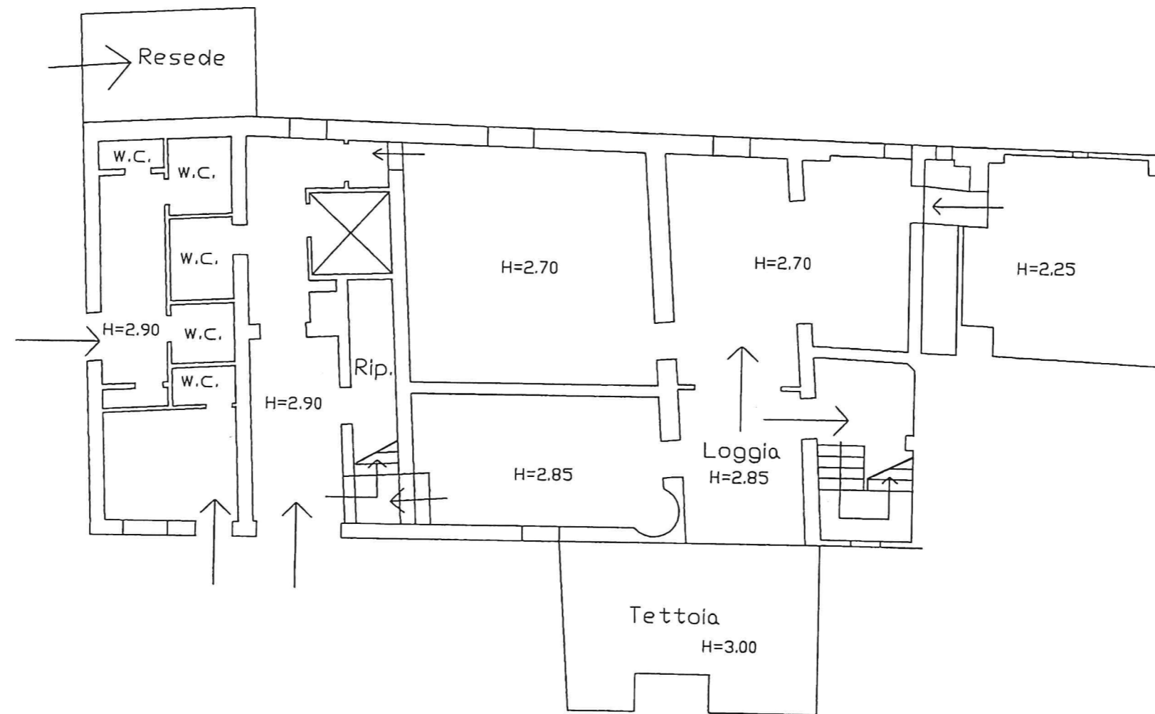
Piano Terra
